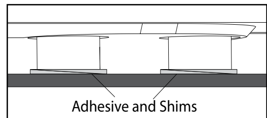
FIGURE 4. If needed, place shims under feet into adhesive to level base.
