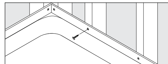
FIGURE 5. If needed, shim between nail flange and stud(s) for tight fit. Screw flange to all studs.
