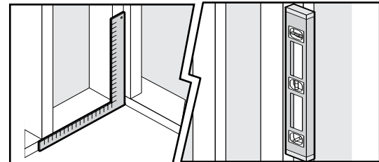
FIGURE 1. Check that studs are plumb with sub-floor/base.
