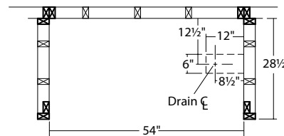
5427 Stud Layout Fits most standard 54" x 27" shower walls. RH drain shown, reverse for LH drain
