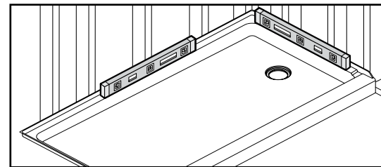
FIGURE 2. Check to assure base is level.
