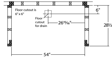
5427 Stud Layout Fits most standard 54" x 27" shower walls.
